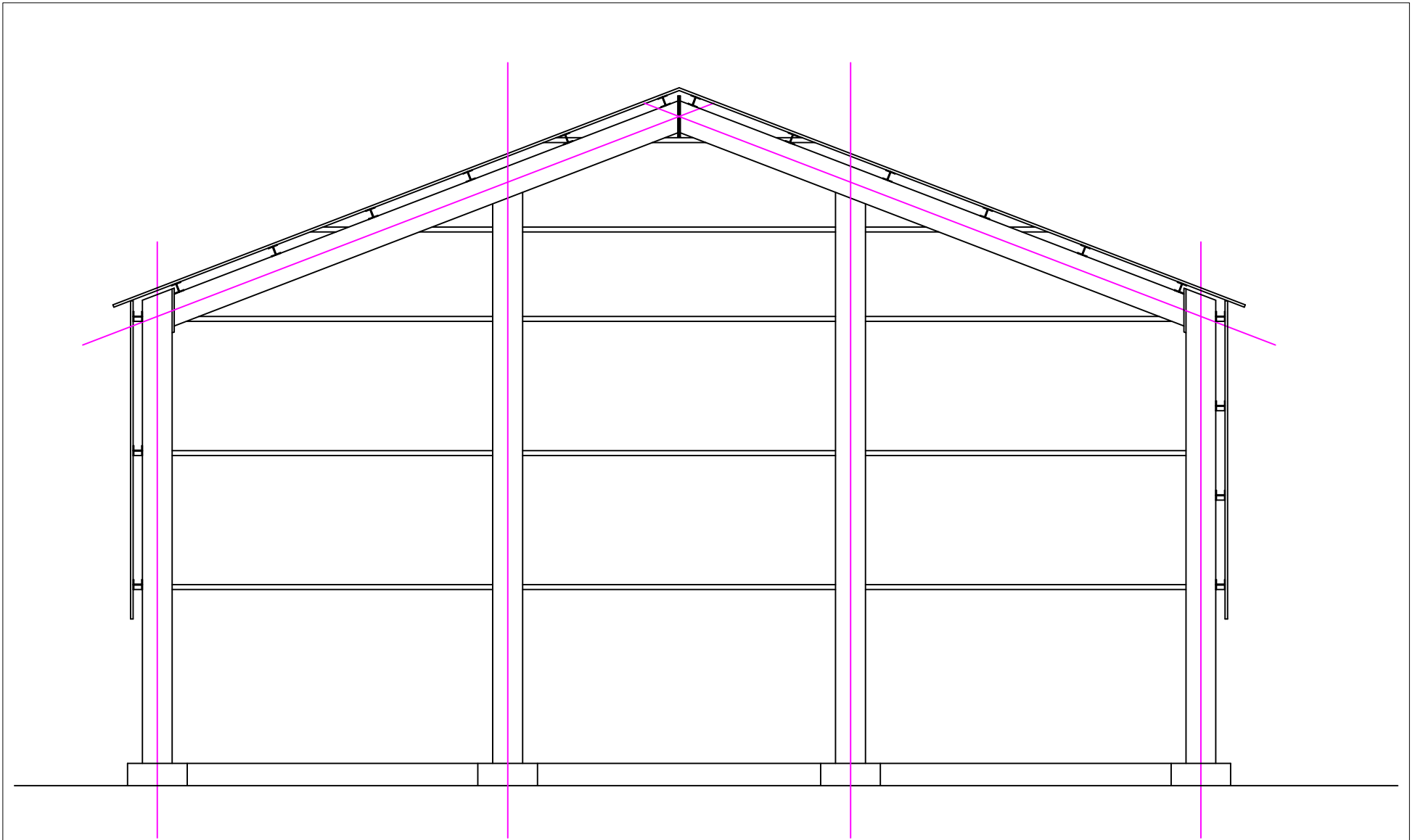
SECTION X-X
