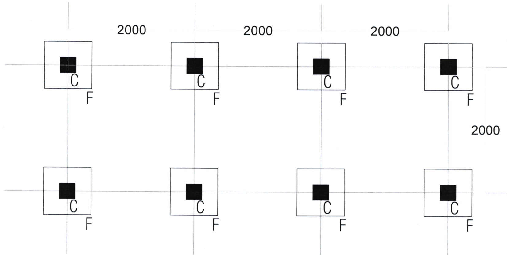
FOOTING AND COLUMN LAYOUT
