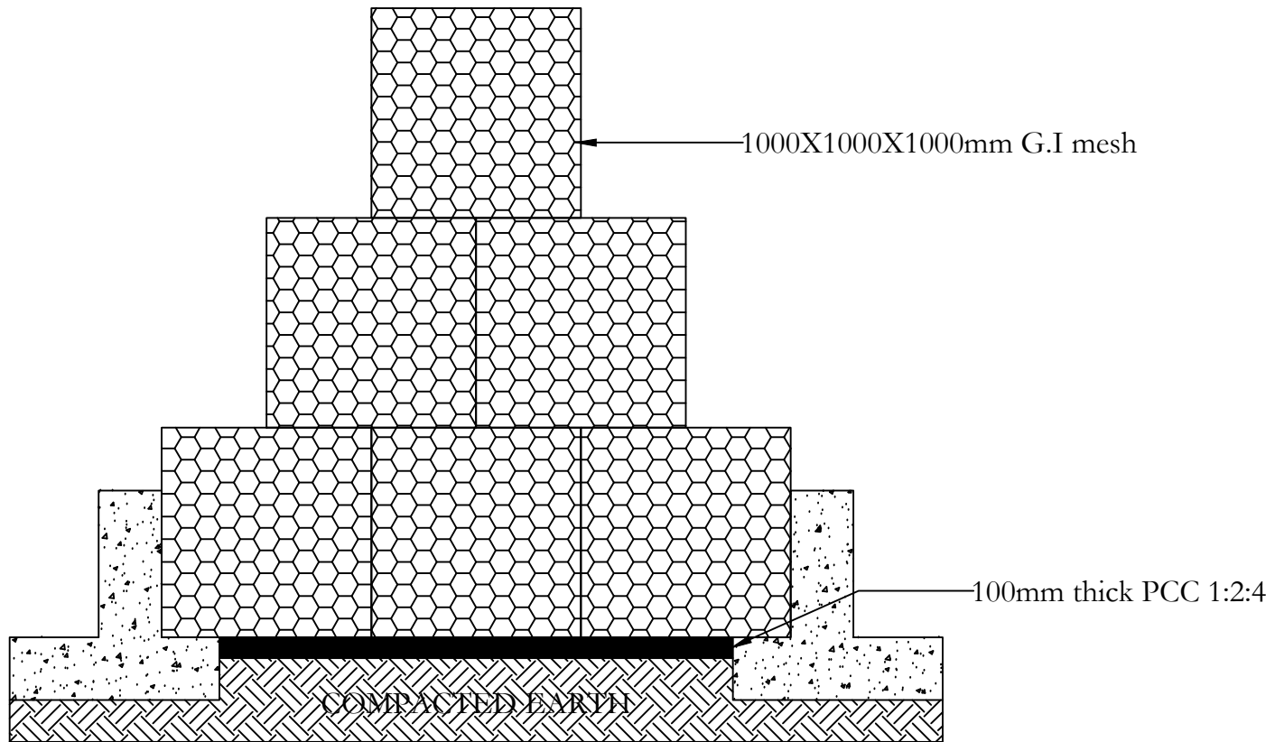
TYPICAL VIEW OF 3m HEIGHT GABION CHECK DAM
