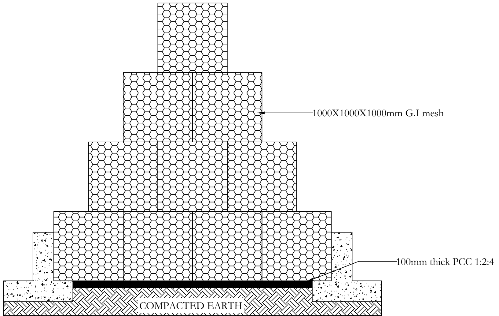
TYPICAL VIEW OF 4m HEIGHT GABION CHECK DAM
